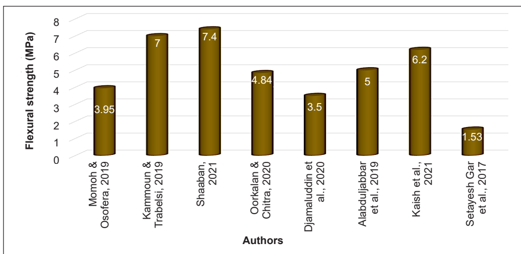
Figure 9. Maximum flexural strength results after 28 days from different studies
