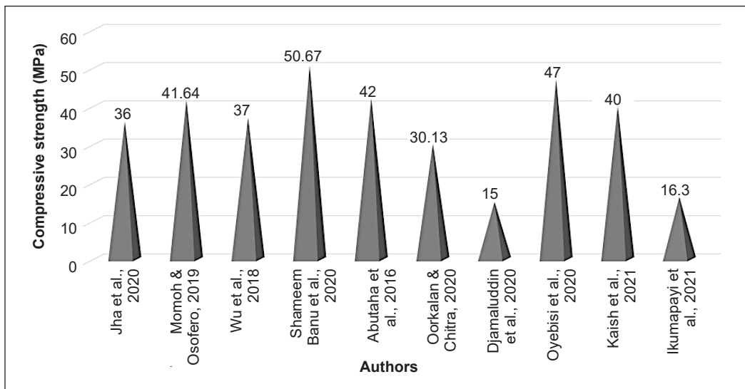
Figure 8. Maximum compressive strength results after 28 days from different studies
