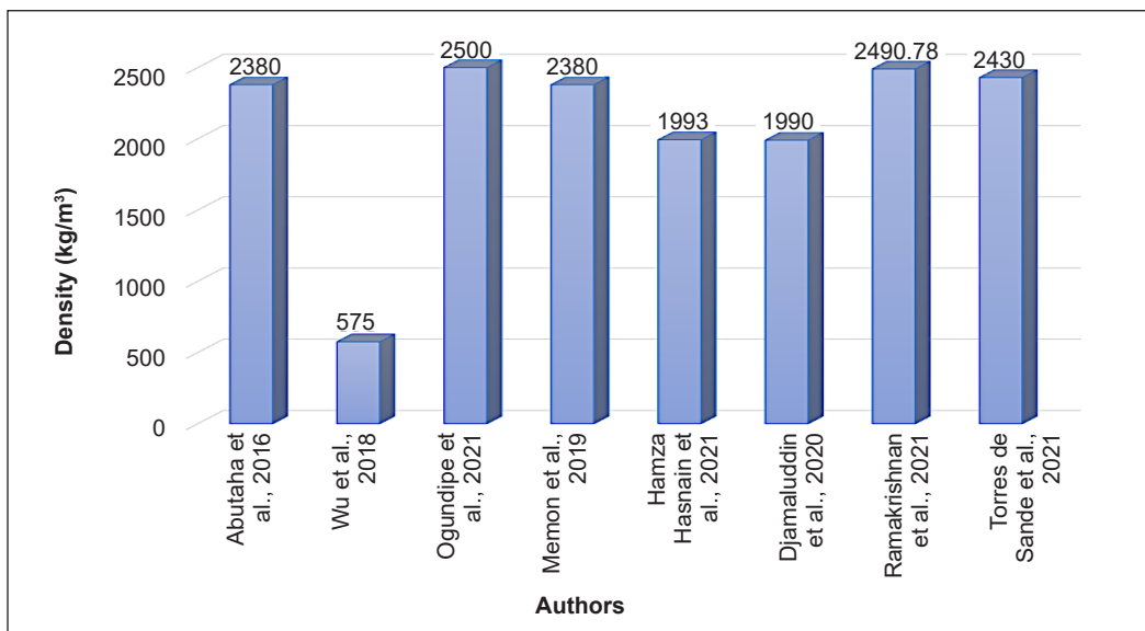
Figure 6. Maximum bulk density results from different studies
