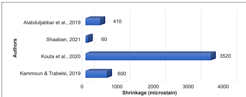
Figure 7. Maximum shrinkage results from different studies
