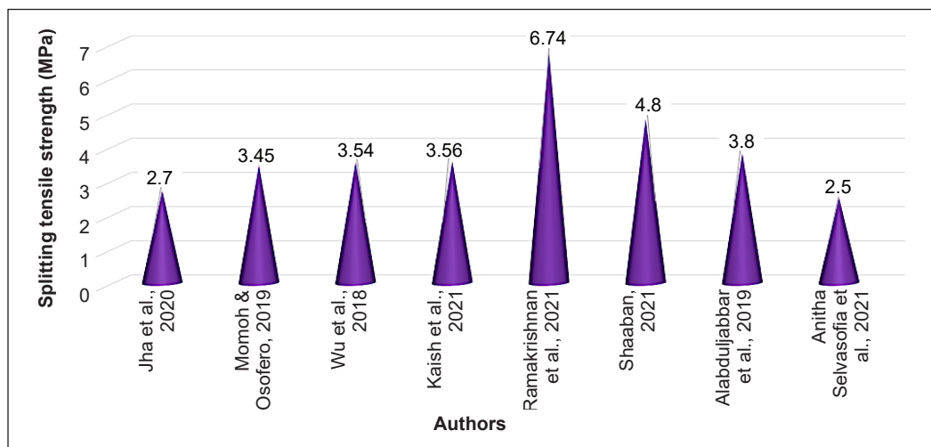
Figure 11. Maximum splitting tensile strength results after 28 days from different studies
