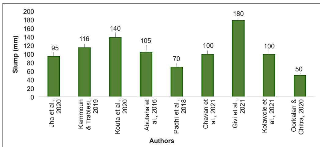
Figure 5. Maximum slump result from different studies
